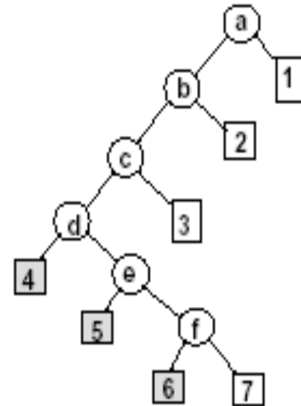
Binary Tree
